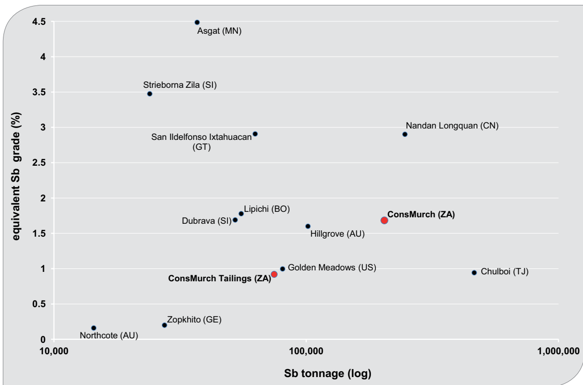
Fig. 5.3.14: Grade-tonnage diagrams (total Sb resources on X-axis) to evaluate the values of different Sb producing mines worldwide. Top: Under consideration with Sb grades only; Bottom: calculation considers other produced commodities: gold, silver (Asgat, Strieborna Zila, Nandan Longquan), copper (Asgat, Strieborna Zila), lead, zinc and tin (Nandan Longquan). Country codes after international standard ISO-3166-ALPHA-2.
