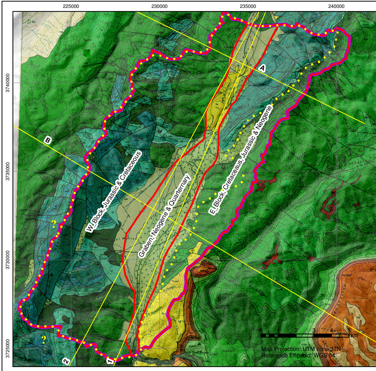
Figure 4-5: Hydrogeologic Blocks
