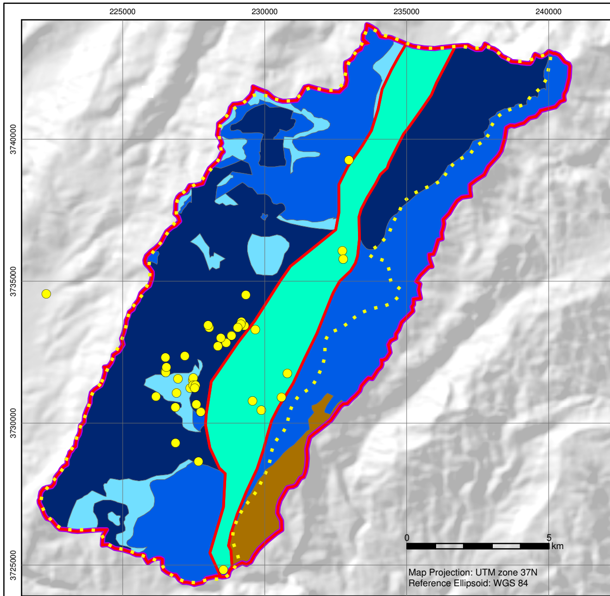
Figure 4-9: Transmissivity Zones
