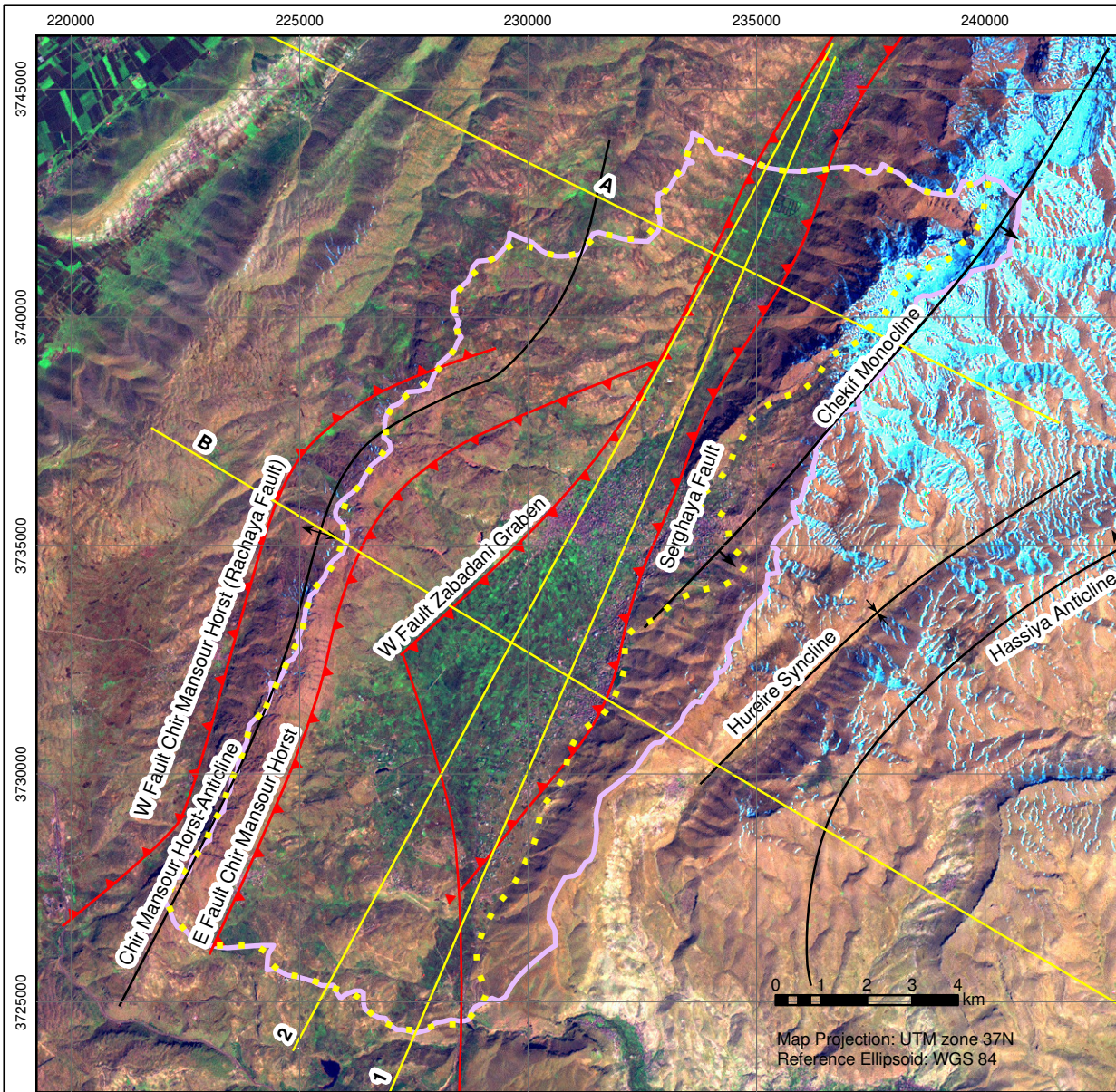
Figure 4-3: Tectonic map
