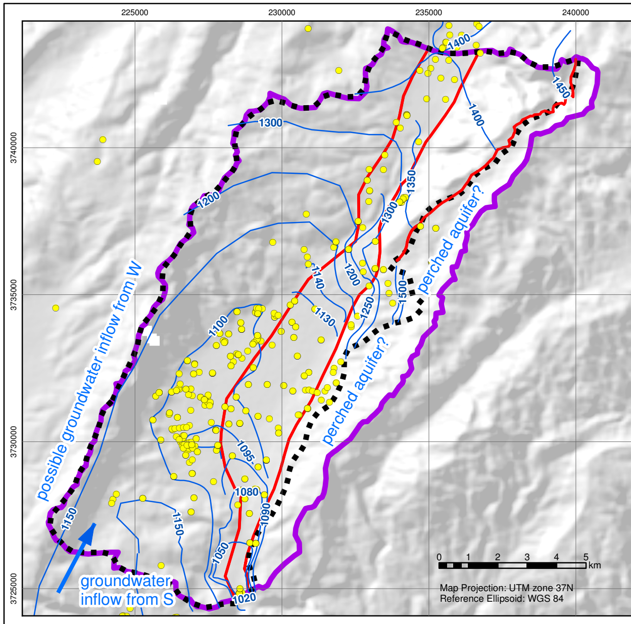
Figure 4-12: Groundwater Contour Map
