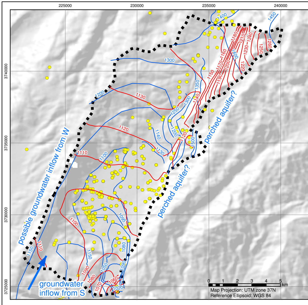
Figure 4-22: Computed versus measured GW-levels
