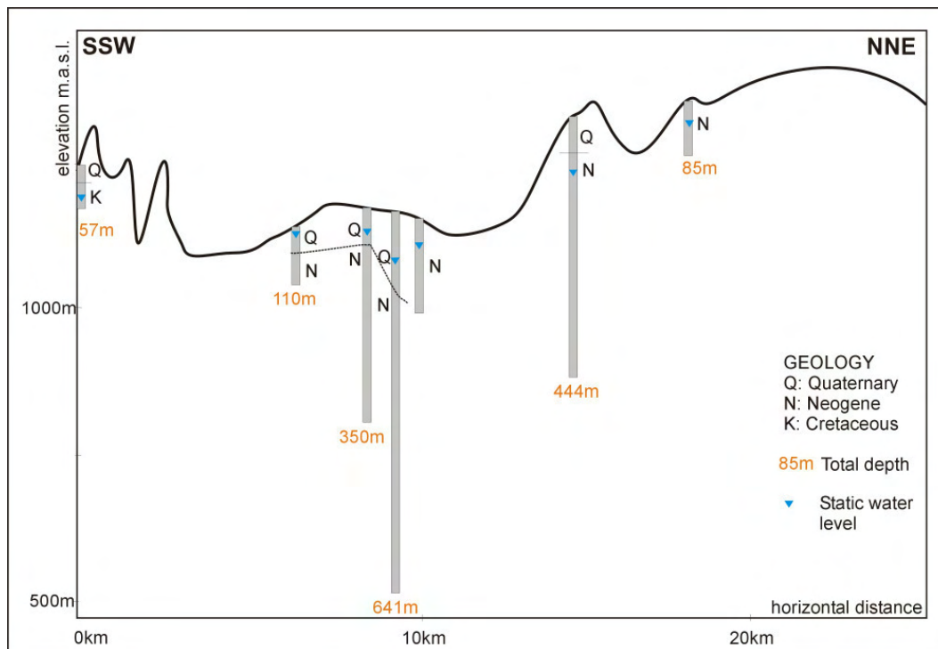
Cross section I, location see Figure 4-5 (borehole data from RUSSIAN STUDY, 1986).
