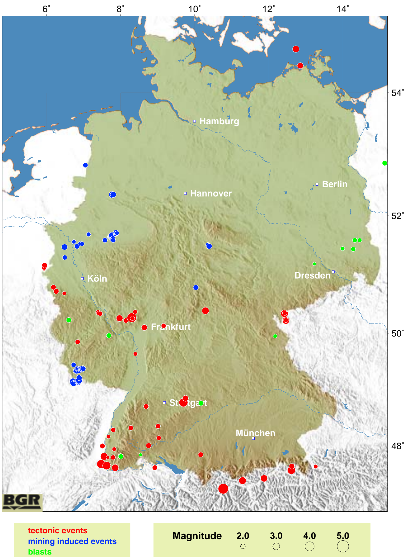
Figure 2: Epicenters of earthquakes in Germany 1997
