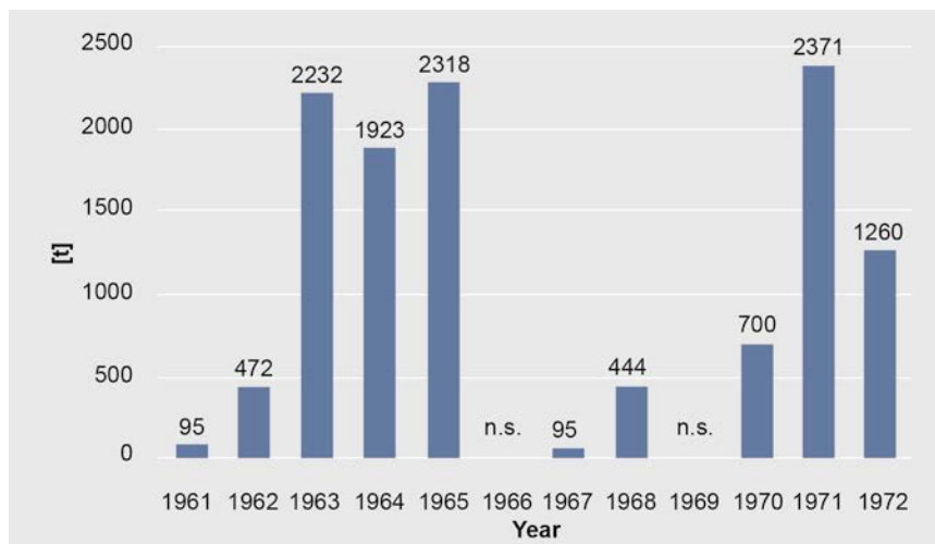
Figure 11: Feldspar production in Namibia in [t] per year (SCHNEIDER 1992).
