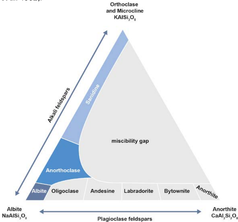
Figure 1: Feldspar triangle indicating solid solution compositions of plagioclases and alkali feldspars feldspars (after DEER et al. 1992).
