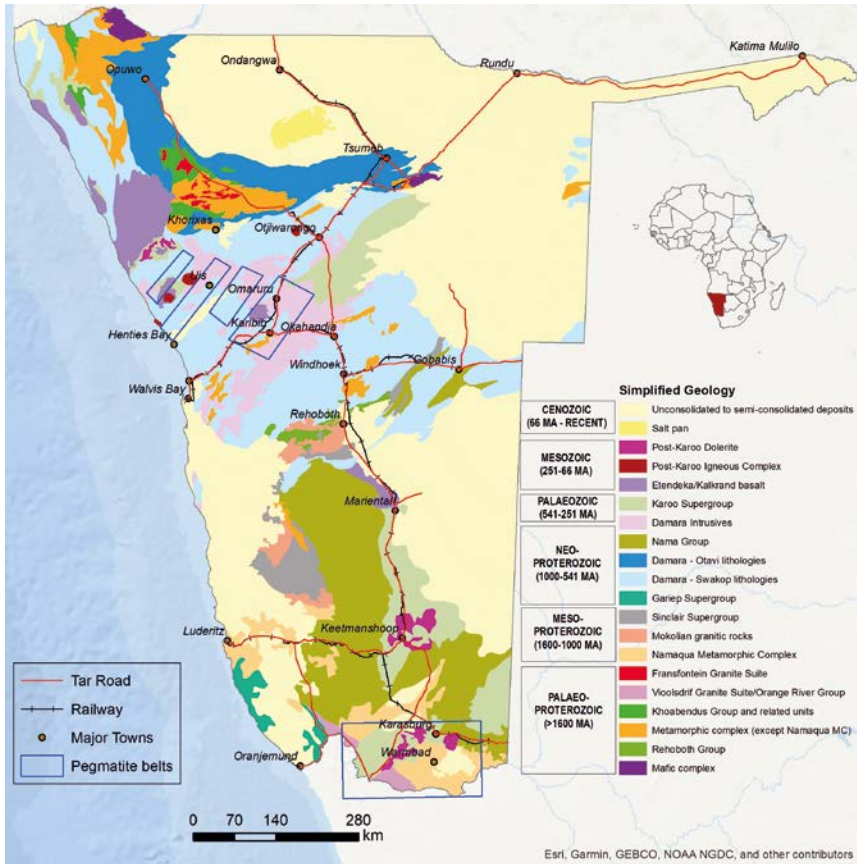
Figure 13: Simplified geology of Namibia with major towns as well as railway and tar roads. Blue polygons indicate pegmatite belts and districts in central and southern Namibia. Data source: GEOLOGICAL SURVEY OF NAMIBIA 2020.
