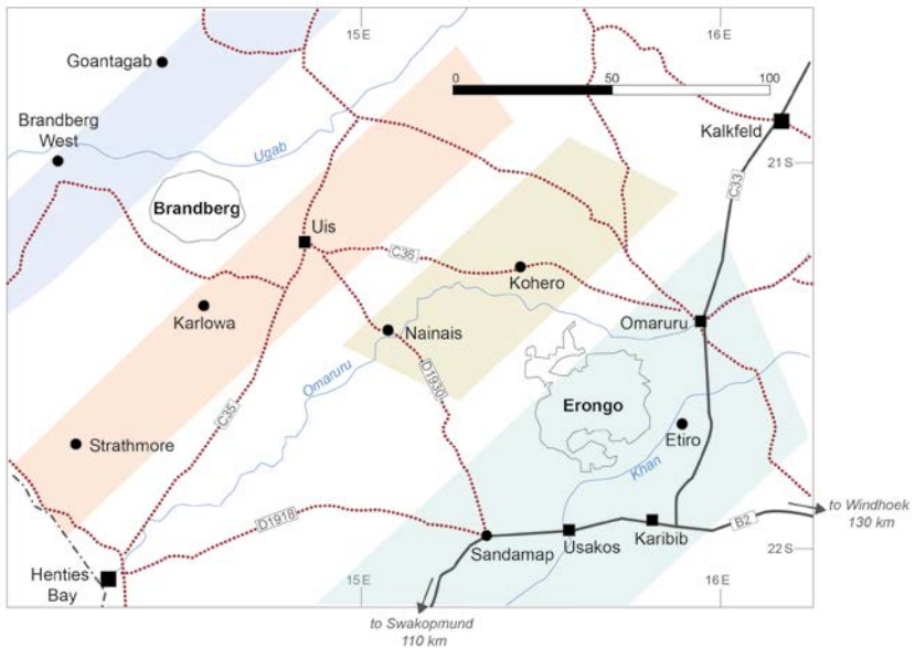
Figure 14: Pegmatite belts in north-central Namibia from west to east: Brandberg West – Goantagab, Cape Cross – Uis, Nainais – Kohero and Sandamap – Erongo as well as the Karibib Pegmatite District after GEOLOGICAL SURVEY OF NAMIBIA (2002).
