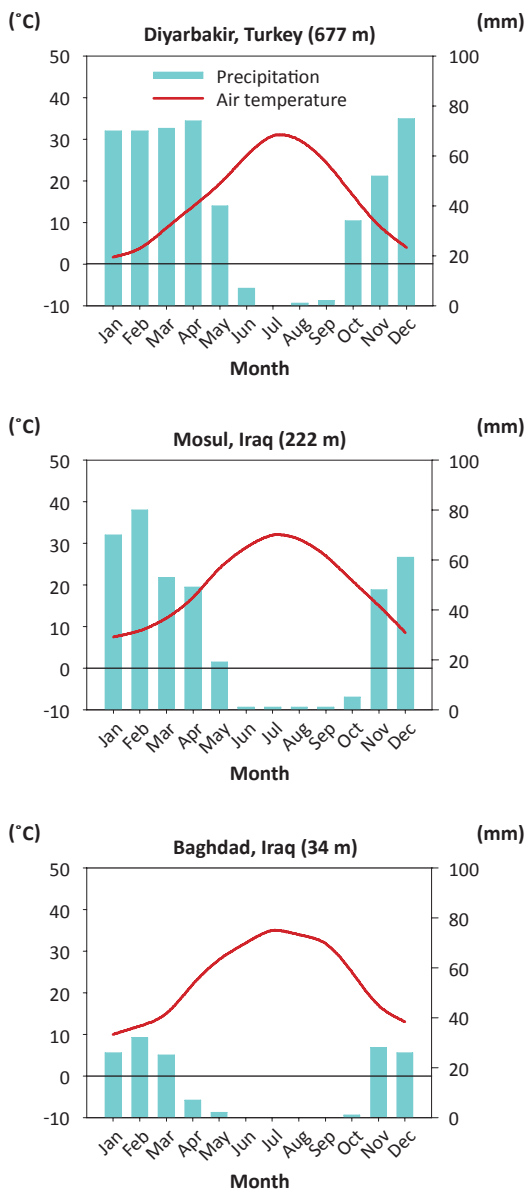
Figure 3. Climate diagrams for Diyarbakir in Turkey, Mosul in Iraq and Baghdad in Iraq
