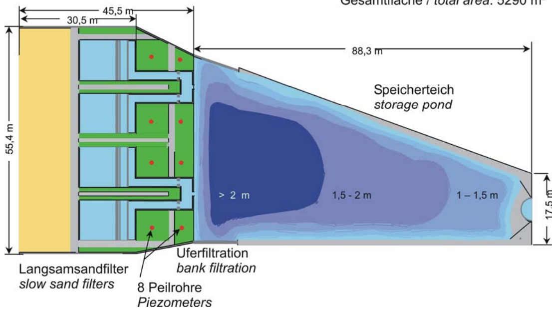
The UBA Experimental Site: map view of the installations for bank filtration.
